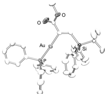
Figure 1. Molecular view of complex 2 in the solid state (thermal ellipsoids set at 50% probability; hydrogen atoms are omitted for clarity). [25]
