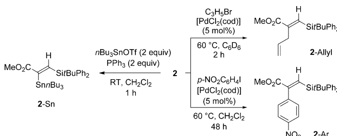
Scheme 3. Functionalization of the \beta -silyl vinylgold complex 2 by transmetalation/cross-coupling. cod = cyclooctadiene.
