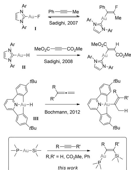
Scheme 1. Reactions of gold fluoride, gold hydride, and gold silyl complexes with alkynes and allenes.
