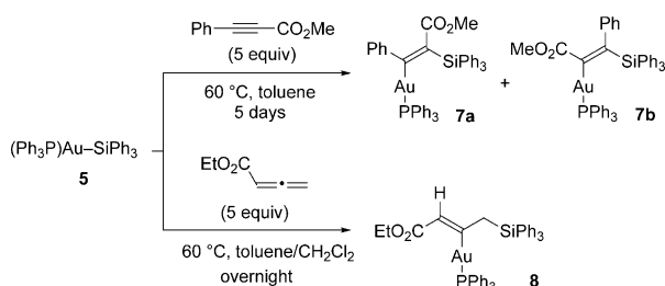
Scheme 5. Alkyne and allene syn insertions in the Au-Si bond of the gold silyl complex 5 .
