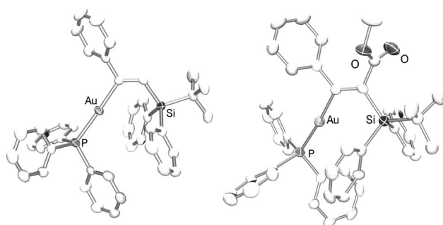
Figure 2. Molecular view of complexes 3 (left) and 4 (right) in the solid state (thermal ellipsoids set at 50% probability; hydrogen atoms and solvent molecules are omitted for clarity). [25]
